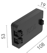
OPTIONAL Power supply Electrical 08.0613.14A Dimmable control box 1-10V, 24/48V. For remote installation.
