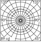
Luminous flux luminaire 1657 lm
