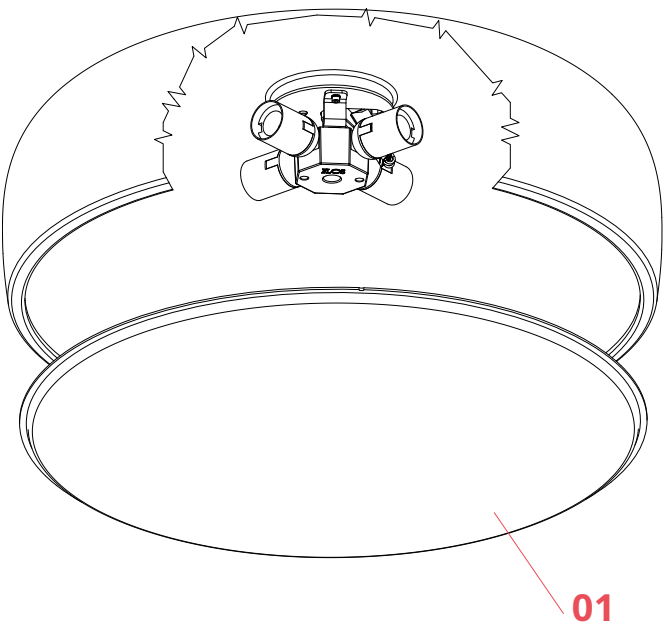
01. Methacrylate diffuser
