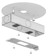
REQUIRED 08.0252.40.19 Surface Spacer
