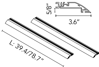
Light Cut Mini 2.75" [70mm] Aluminum profile is adapted to 5/8" ceiling thickness
