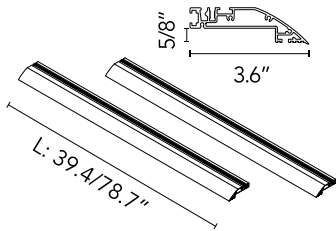
Light Cut Mini 2.75" [70mm] Aluminum profile is adapted to 5/8" ceiling thickness
