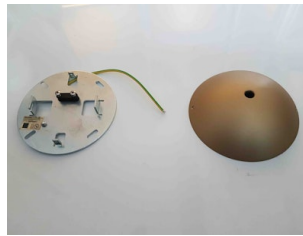
RFU317359 Suspension 1/Suspension 2 Brass Ceiling Rose Assembly
