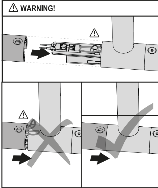
ENDCAP
